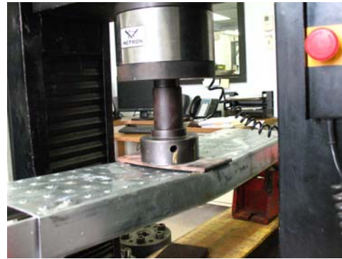
Point load failure at 4,435 lbs.
