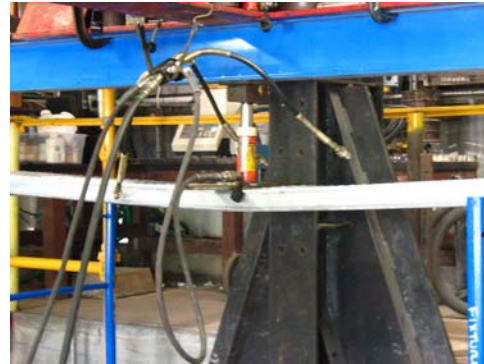
Point load failure at 1,525 bs.
