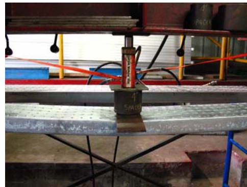
Point load failure at 2,275 lbs.
