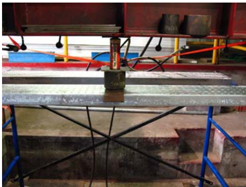
Point load setup
